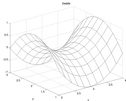
Fig. 9: Plot of Saddle function.
