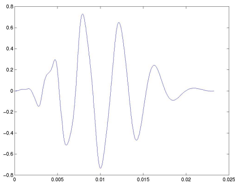
Fig. 12: Graph of “sound data” from Example 24.1
